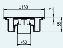
PV DN 50/55 B (PV DN 50/84)
